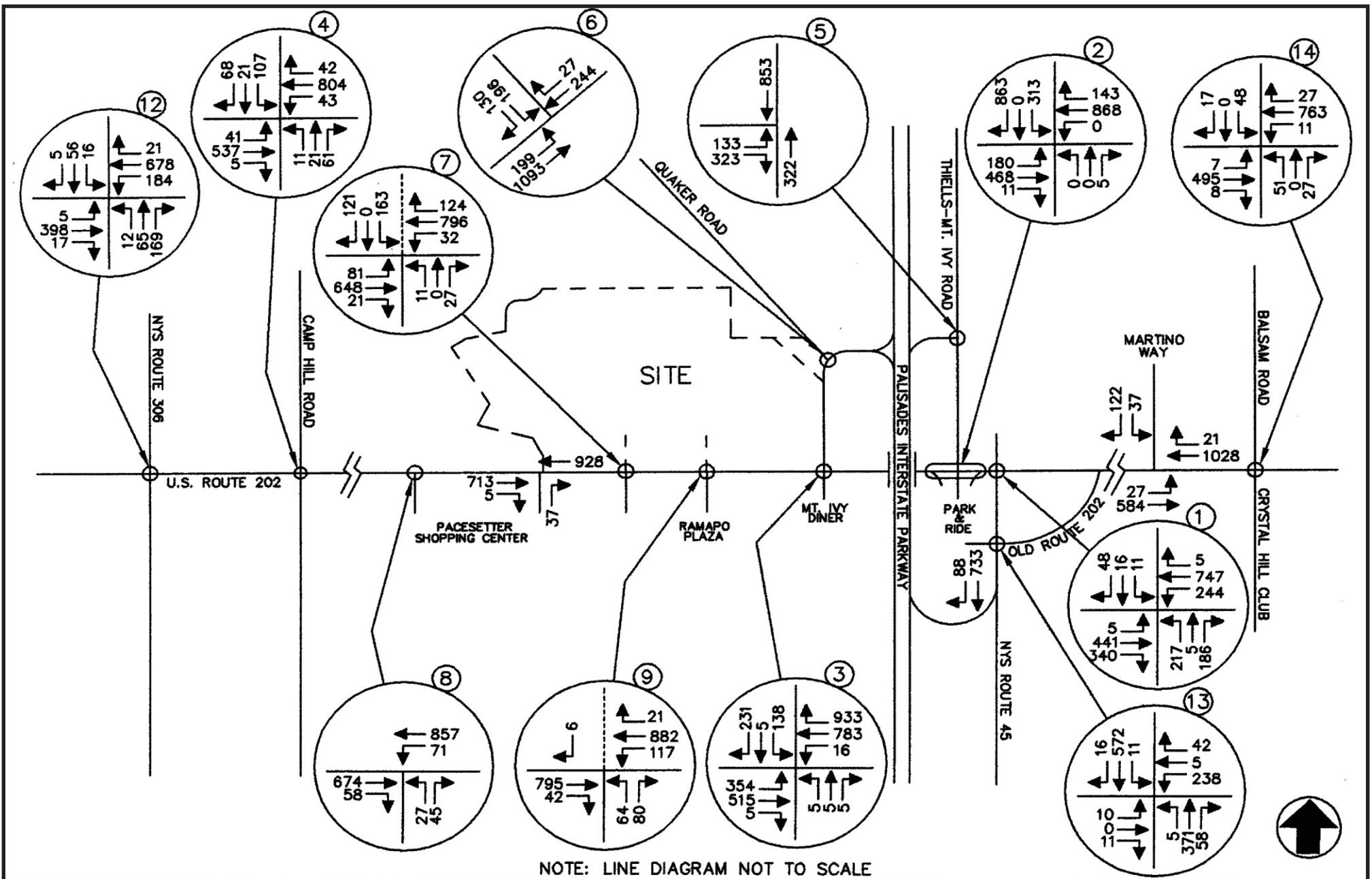
Figure 3.5-33: 2011 Build Traffic Volumes Weekday Peak AM Highway Hour (With Patrick Farm) Minisceongo Park Towns of Haverstraw & Ramapo, Rockland County, New York Source: John Collins Engineers, P.C. Date: October, 2008
